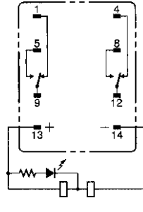
MY4(Z)N/MY4(Z)IN (DC Models)
