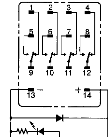
MY4(Z)N-D/MY4(Z)IN-D2 (DC Models Only)
