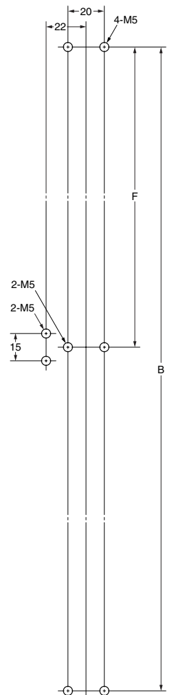
Mounting screw holes
