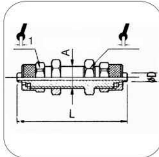
ART. 304 Raccordo intermedio passaparete Bulkhead connector
