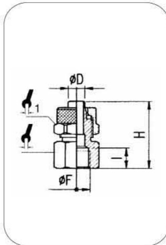
ART. 302 Raccordo diritto femmina Straight female adaptor
