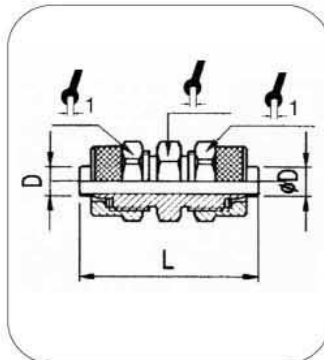
ART. 303 Raccordo diritto intermedio Straight connector
