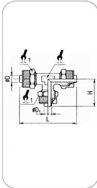
ART. 309 Raccordo T intermedio Tee connector
