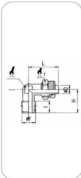
ART. 305 Raccordo ad L maschio conico Elbow taper male adaptor
