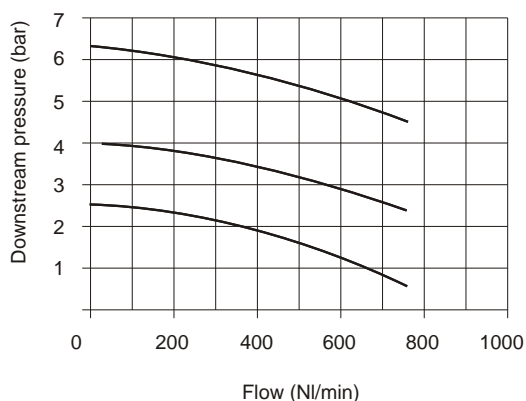
Adjustment characteristics
