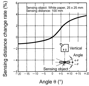
E3S-LS10 (Vertical Direction)
