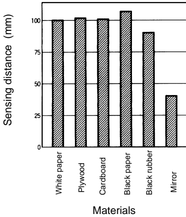
Sensing of White Paper at a Setting Distance of 100 mm
