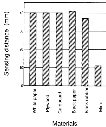
Sensing of White Paper at a Setting Distance of 40 mm
