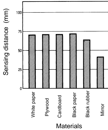
Sensing of White Paper at a Setting Distance 70 mm
