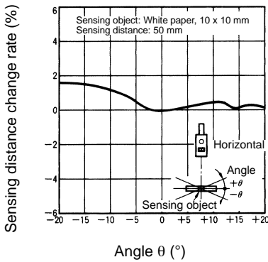
E3S-LS5 (Horizontal Direction)
