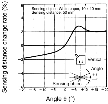
E3S-LS5 (Vertical Direction)
