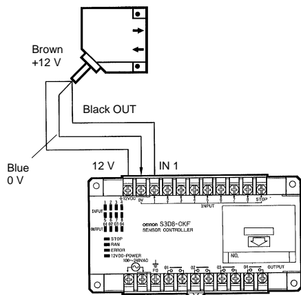
With S3D8 Sensor Controller
