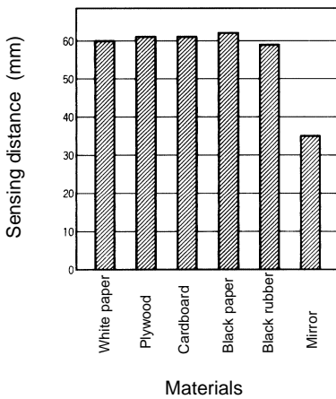
Sensing of White Paper at a Setting Distance of 60 mm
