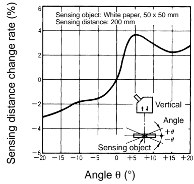
E3S-LS20 (Vertical Direction)
