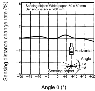
E3S-LS20 (Horizontal Direction)
