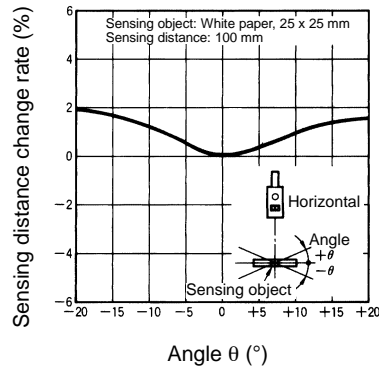
E3S-LS10 (Horizontal Direction)
