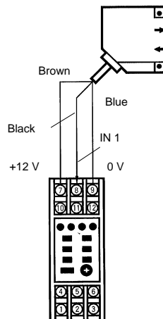
With S3D2 Sensor Controller
